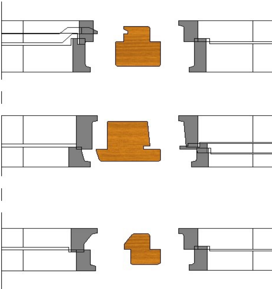
WINDOW PROFILE EXAMPLE
