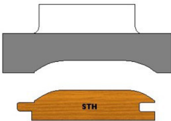
LOG PANEL STH. CUTTER LENGHT 125 MM
