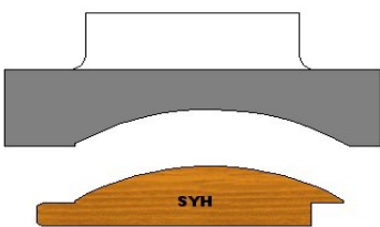
LOG PANEL SYH. CUTTER LENGHT 125 MM
